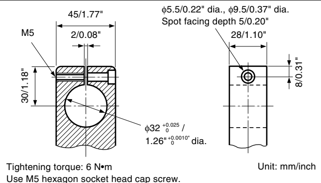
Fig. 2 Mount holder dimensions
